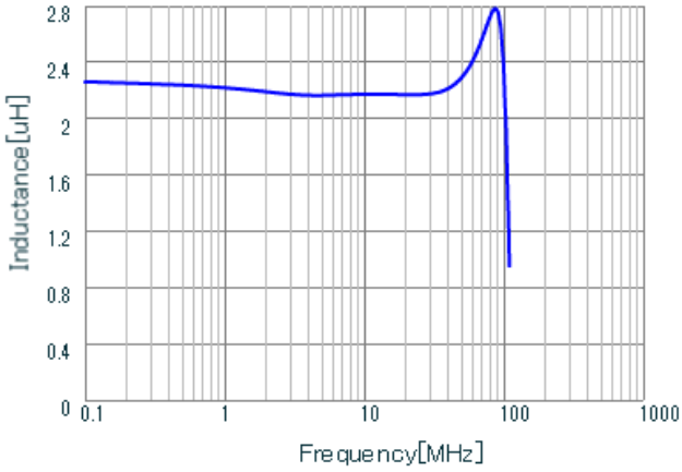
LQH44PN2R2MJ0 L
