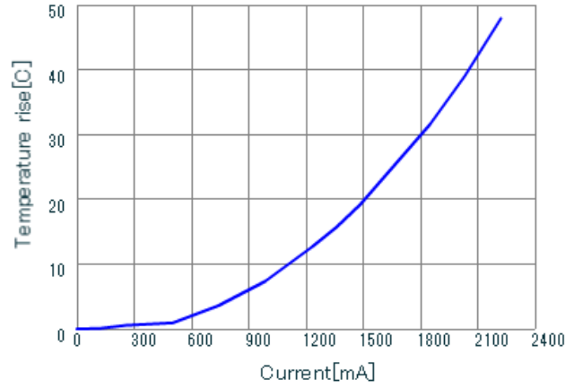
LQH44PN2R2MJ0 DT_Current
