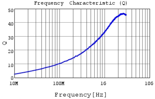
LQG15HH2N2S02 Q
