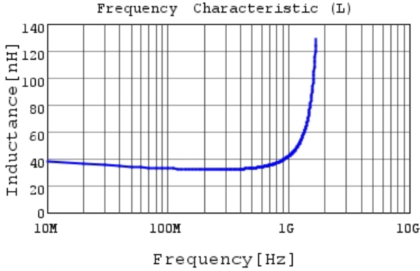
LQG15HS33NJ02 L
