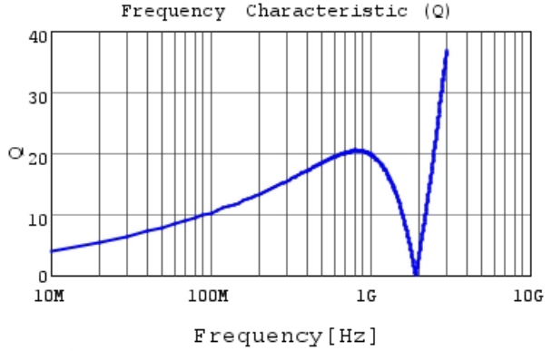
LQG15HS33NJ02 Q
