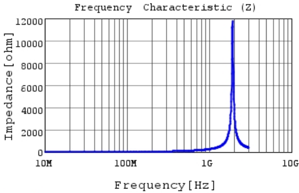
LQG15HS33NJ02 |Z|
