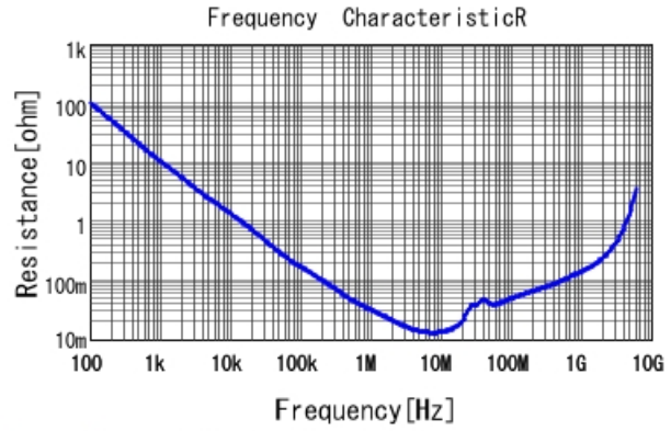
GRM188R61E474KA12 R DCOV, 25degC
