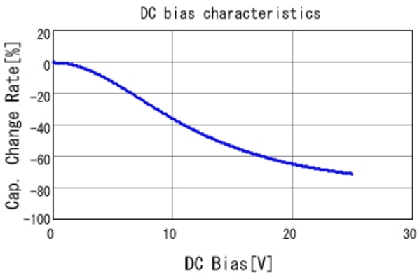
GRM188R61E474KA12 C-DC bias capchange, 25.0degC, A
