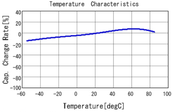
GRM188R61E474KA12 C-Temp. capchange, DC0.0V, AC1.C
