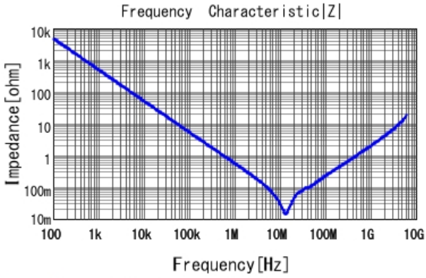
GRM188R61E474KA12 |Z| DCOV, 25degC
