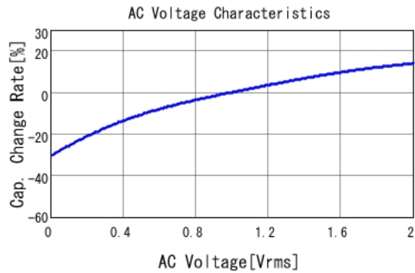
GRM188R61E474KA12 C-AC Voltage capchange, DCOV, 25
