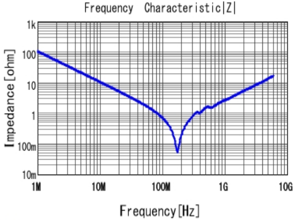
■ GRM1882C2A152JA01 |Z| DCOV, 20degC
