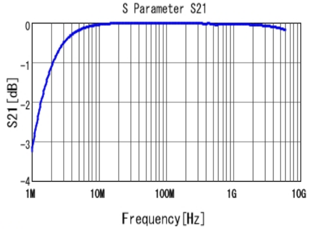
■ GRM1882C2A152JA01 S21 DCOV, 20degC
