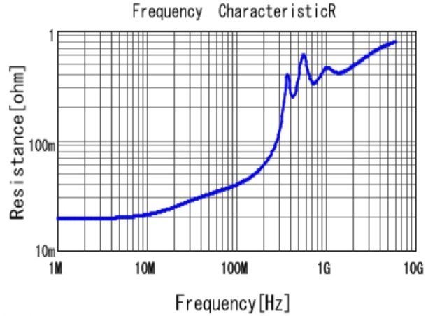
■ GRM1882C2A152JA01 R DCOV, 20degC
