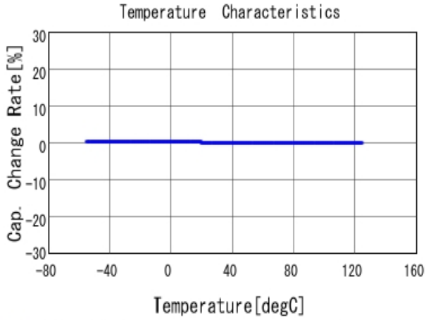
■ GRM1882C2A152JA01 C-Temp. capchange, DCOV, AC1Vrms
