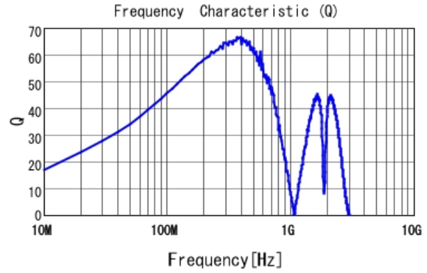
LQW2BANR20J00 Q
