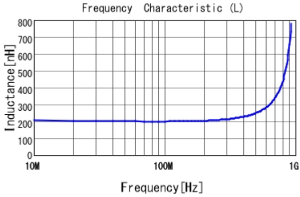
LQW2BANR20J00 L
