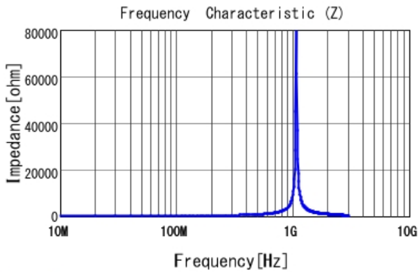
LQW2BANR20J00 |Z|
