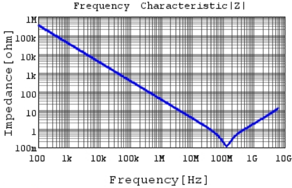
GRM155R71H472KA01 |Z| DCOV, 25degC
