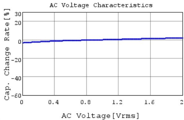
GRM155R71H472KA01 C-AC Voltage capchange, Dc
