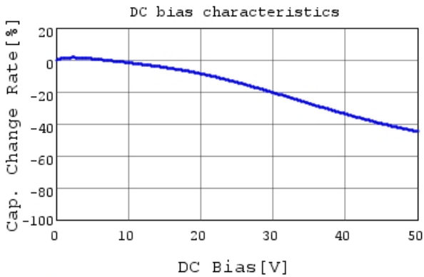
GRM155R71H472KA01 C-DC bias capchange, 25.0c
