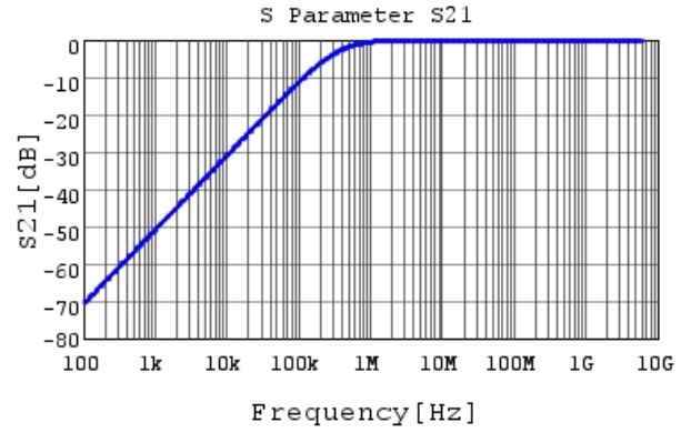
GRM155R71H472KA01 S21 DC0V, 25degC
