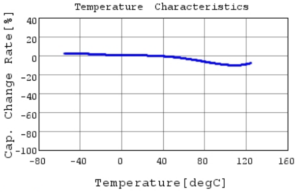
GRM155R71H472KA01 C-Temp. capchange, DC0.0V,
