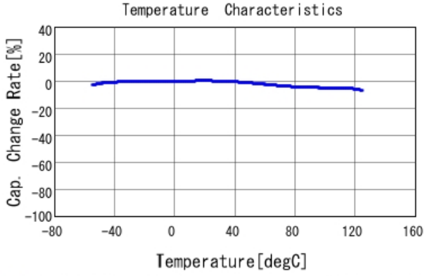
■ GCE188R71H103KA01 C-Temp. capchange, DCO. 0V, AC1. 0Vrm
