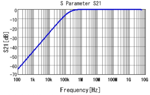
■ GCE188R71H103KA01 S21 DCOV, 25degC
