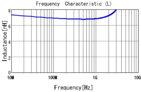
LQW15AN7N0G00 L
