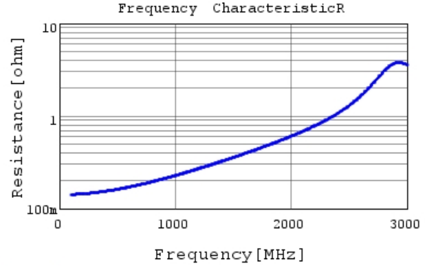
GRM31A5C2J560JW01 R DC0V, 25degC
