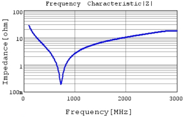
GRM31A5C2J560JW01 |Z| DC0V, 25degC
