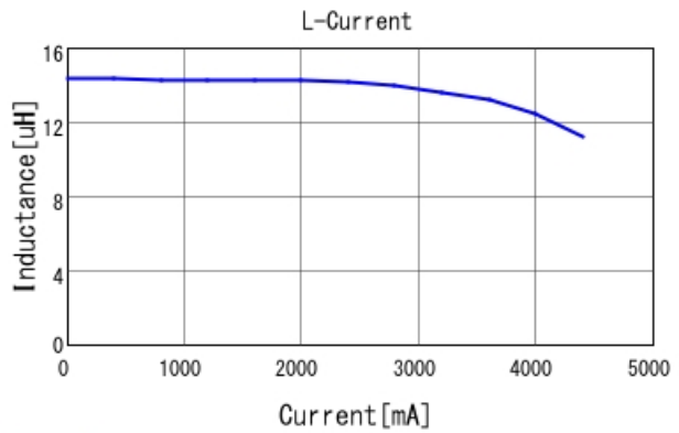
#B952AS-H-150M=P3 L-Current 20degC
