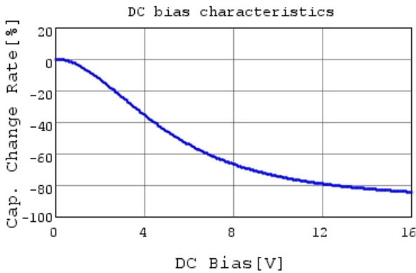
GRM155R61C225KE11 C-DC bias capchange, 25.0c
