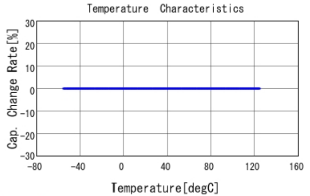
GRM21A5C2E471JWA1 C-Temp. capchange, DCOV, AC1Vrms
