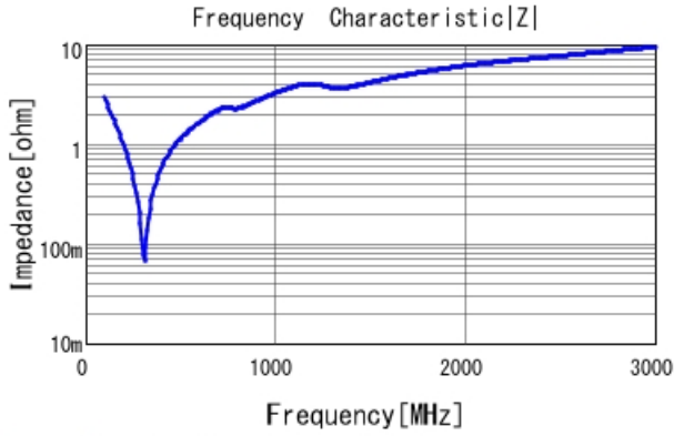
GRM21A5C2E471JWA1 |Z| DCOV, 25degC
