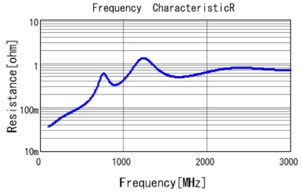
GRM21A5C2E471JWA1 R DCOV, 25degC
