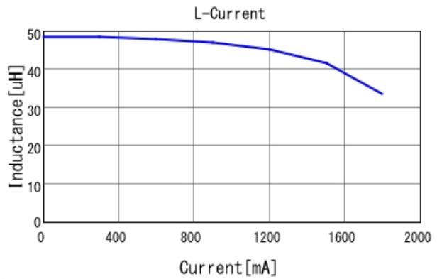
1273AS-H-470M L-Current 20degC
