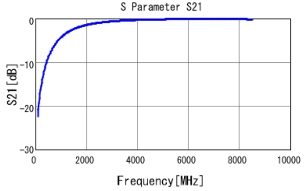
GRM1555C1H1R2CA01 S21 DCOV, 25degC
