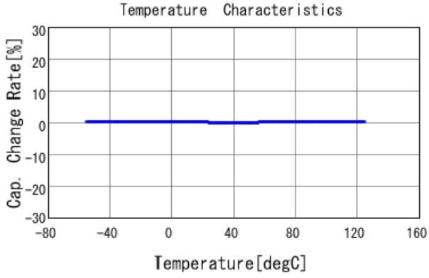
GRM1555C1H1R2CA01 C-Temp. capchange, DCOV, AC1Vrms
