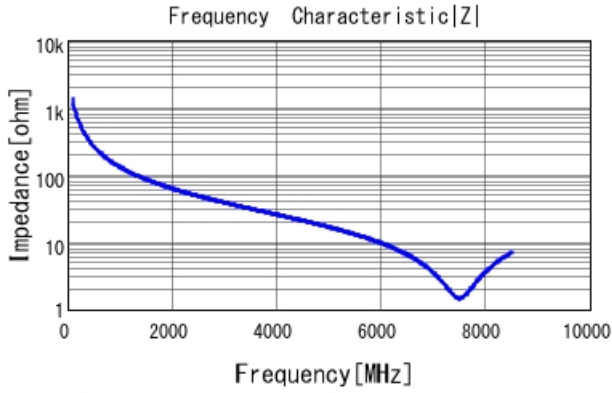
GRM1555C1H1R2CA01 |Z| DCOV, 25degC
