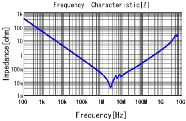
GRM32DR11E475KA61 |Z| DCOV, 20degC
