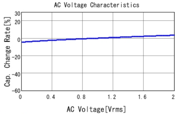
GRM32DR11E475KA61 C-AC Voltage capchange, DCOV, 2C
