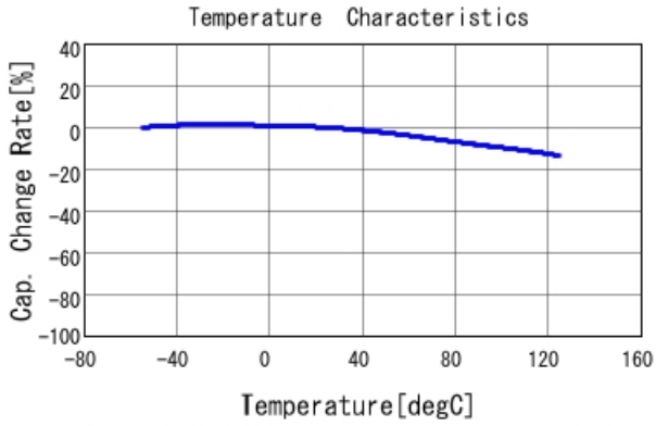
GRM32DR11E475KA61 C-Temp. capchange, DC0.0V, AC1.C
