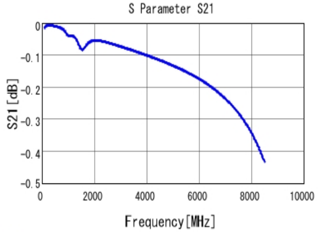
■ GRM1552C1H331JA01 S21 DCOV, 20degC
