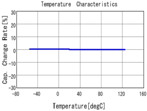
■ GRM1552C1H331JA01 C-Temp. capchange, DCOV, AC1Vrms
