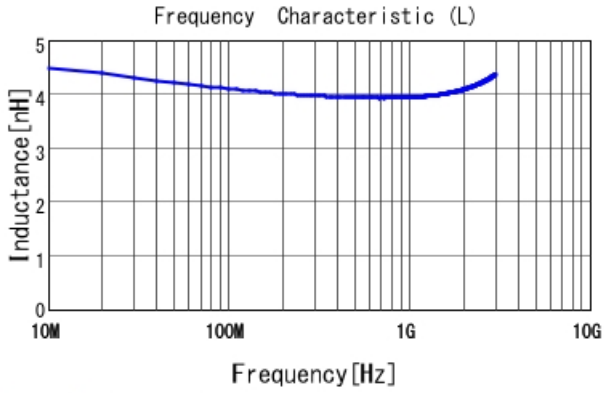
LQP03TQ3N9B02 L
