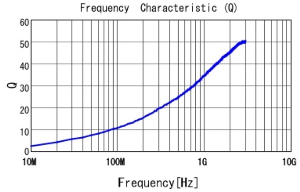
LQP03TQ3N9B02 Q
