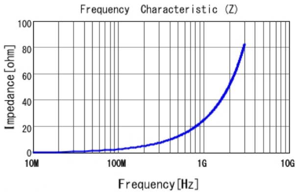
LQP03TQ3N9B02 |Z|
