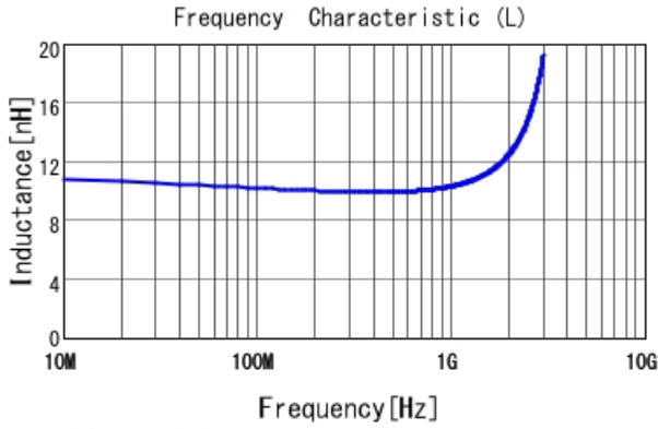
LQG15WZ10NJ02 L
