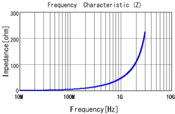
LQG15HN7N5G02 |Z|
