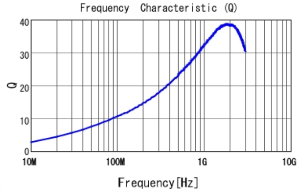
LQG15HN7N5G02 Q
