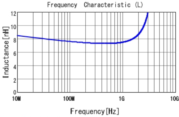
LQG15HN7N5G02 L
