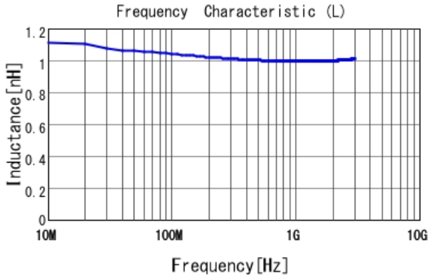
LQP03TN1N0B02 L
