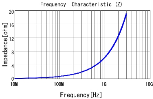
LQP03TN1N0B02 |Z|
