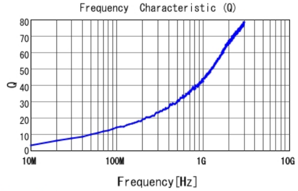
LQP03TN1N0B02 Q
