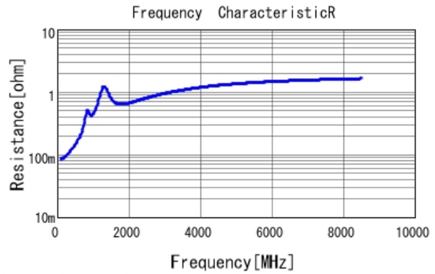
GRM1885C1H331JA01 R DCOV, 25degC
