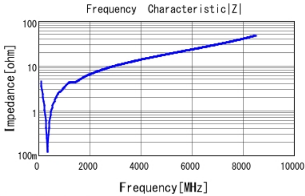
GRM1885C1H331JA01 |Z| DCOV, 25degC
