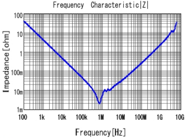
■ GRM32ER61A476KE20 |Z| DCOV, 25degC
