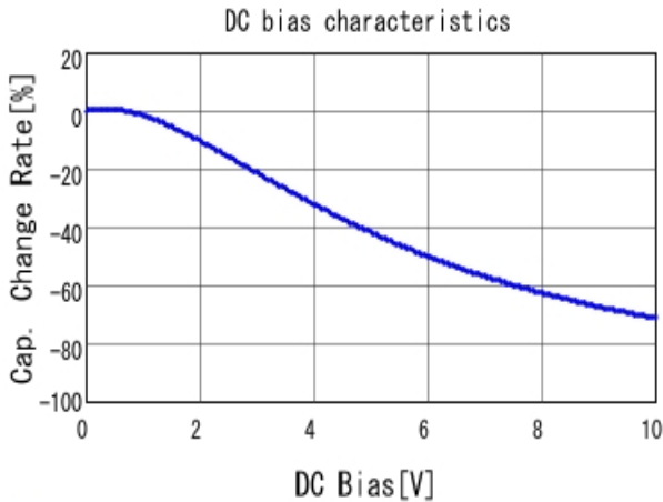
■ GRM32ER61A476KE20 C-DC bias capchange, 25.0degC, AC0.
