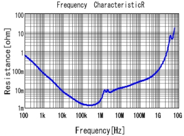
■ GRM32ER61A476KE20 R DCOV, 25degC
