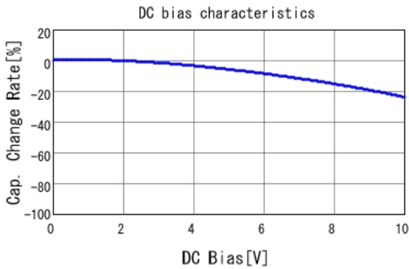
GRM155R71A104KA01 C-DC bias capchange, 25.0degC, A
