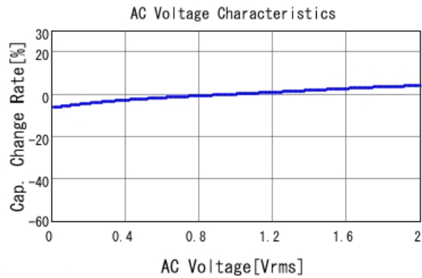
GRM155R71A104KA01 C-AC Voltage capchange, DCOV, 25
