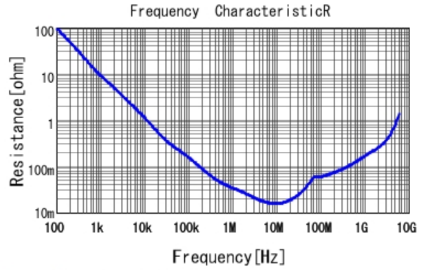
GRM155R71A104KA01 R DCOV, 25degC
