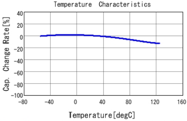
GRM155R71A104KA01 C-Temp. capchange, DC0.0V, AC1.C
