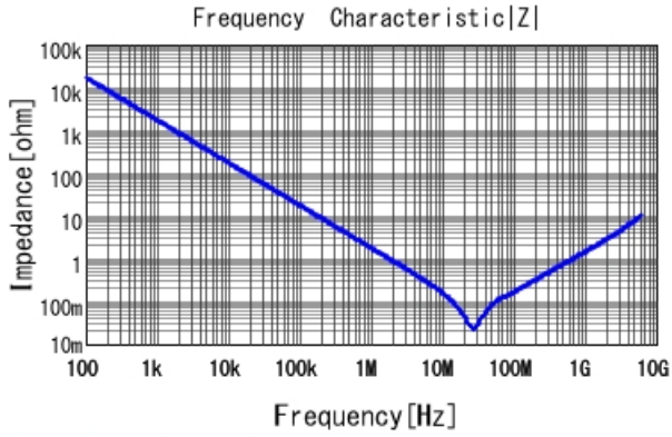
GRM155R71A104KA01 |Z| DCOV, 25degC
