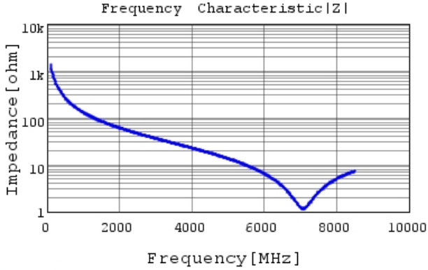
GCM1555C1H1R2BA16 |Z| DCOV, 25degC
