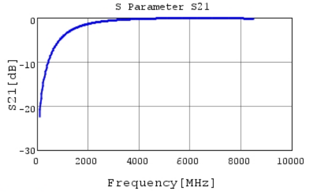
GCM1555C1H1R2BA16 S21 DCOV, 25degC
