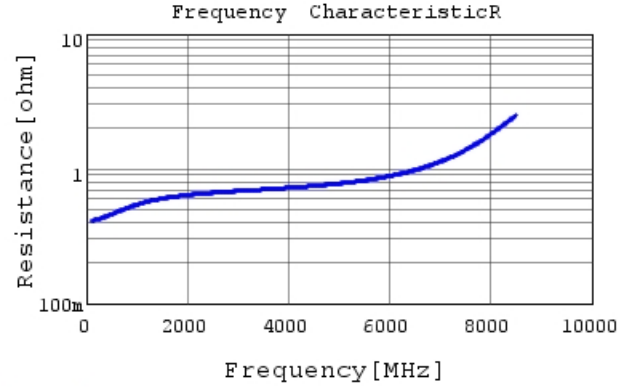
GCM1555C1H1R2BA16 R DCOV, 25degC
