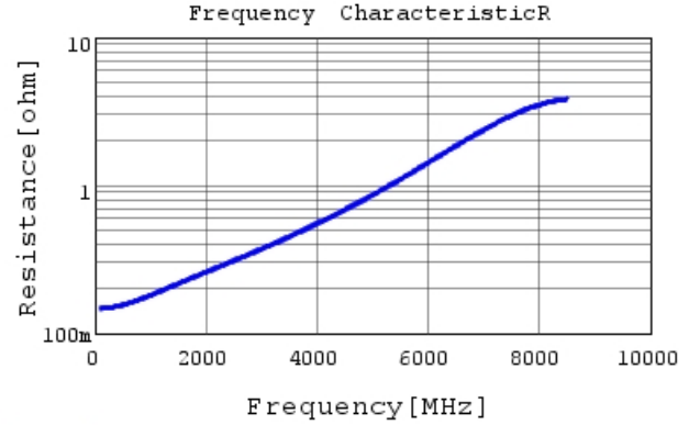
GRM0335C1H330GA01 R DCOV, 25degC
