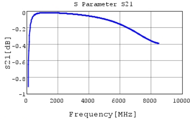
GRM0335C1H330GA01 S21 DCOV, 25degC
