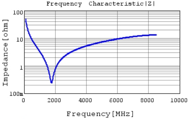
GRM0335C1H330GA01 |Z| DCOV, 25degC
