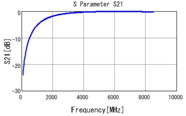
GCM1885C2A1R0BA16 S21 DCOV, 25degC
