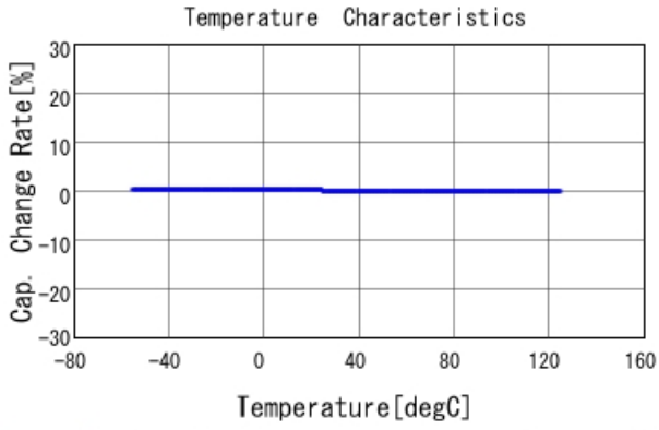
GRM0335C1E8R2CA01 C-Temp. capchange, DCOV, AC1Vrms
