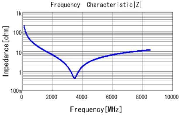
GRM0335C1E8R2CA01 |Z| DCOV, 25degC
