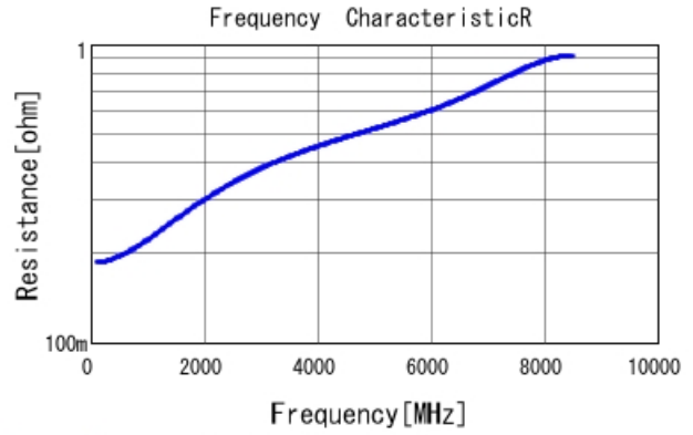
GRM0335C1E8R2CA01 R DCOV, 25degC
