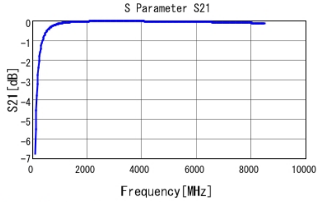
GRM0335C1E8R2CA01 S21 DCOV, 25degC
