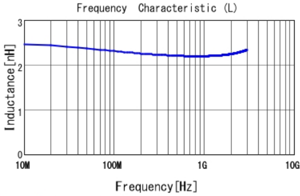
LQP03TN2N2B02 L
