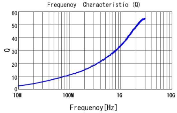
LQP03TN2N2B02 Q
