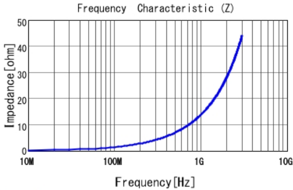
LQP03TN2N2B02 |Z|
