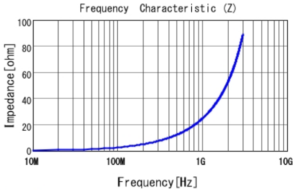
LQP03TG3N9B02 |Z|
