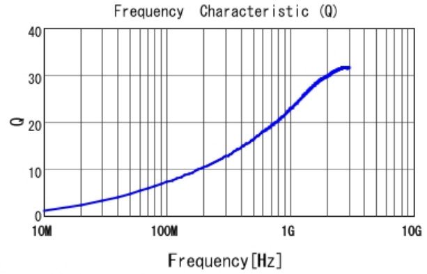
LQP03TG3N9B02 Q
