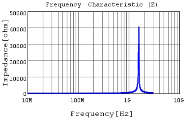
LQW2UAS56NF00 |Z|
