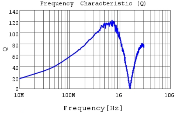
LQW2UAS56NF00 Q
