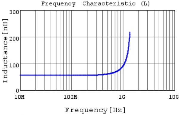
LQW2UAS56NF00 L
