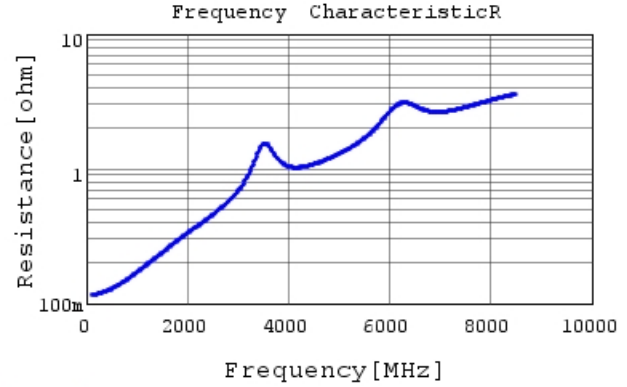
GRT1555C2A270JA02 R DC0V, 25degC
