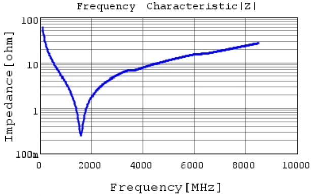
GRT1555C2A270JA02 |Z| DC0V, 25degC
