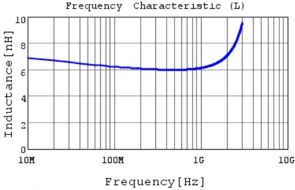
LQG15HN6N2S02 L
