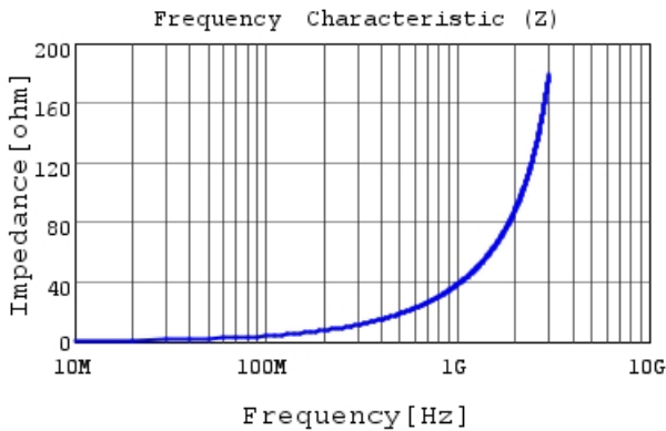
LQG15HN6N2S02 |Z|
