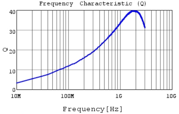
LQG15HN6N2S02 Q
