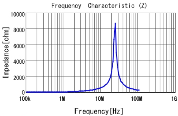
LQH5BPN6R8M38 |Z|
