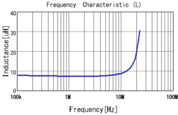
LQH5BPN6R8M38 L
