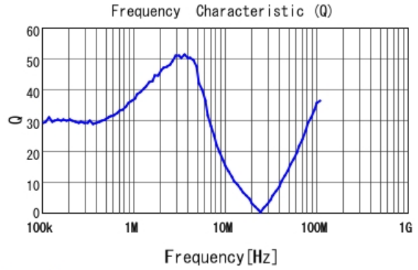
LQH5BPN6R8M38 Q
