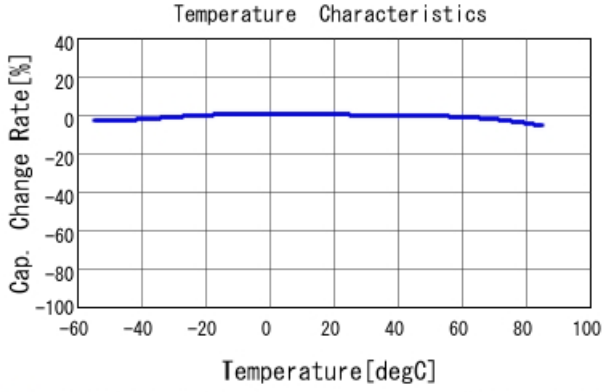
■ GRM21BR61H475ME51 C-Temp. capchange, DCO. 0V, AC1. 0Vrm
