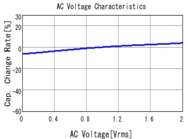
■ GRM32DC72A475KE01 C-AC Voltage capchange, DCOV, 25.0d
