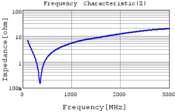
GRM31A5C2J221JW01 |Z| DCOV, 25degC
