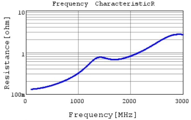
GRM31A5C2J221JW01 R DCOV, 25degC
