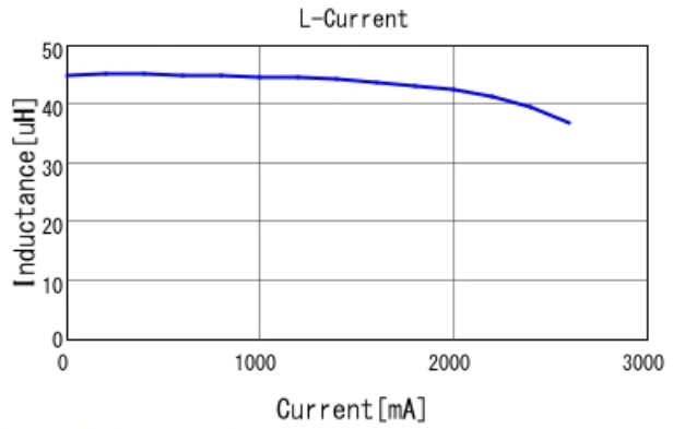
#B952AS-H-470M=P3 L-Current 20degC
