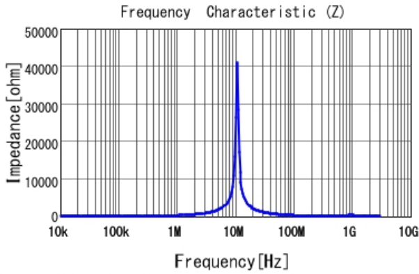
#B952AS-H-470M=P3 |Z|
