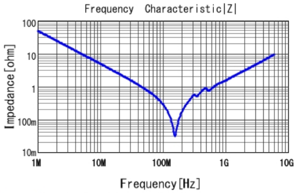
GRM1555C1H332JE01 |Z| DCOV, 25degC
