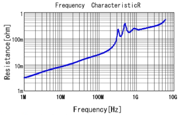
GRM1555C1H332JE01 R DCOV, 25degC
