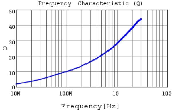
LQP03TN3N4BZ2 Q
