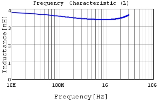
LQP03TN3N4BZ2 L
