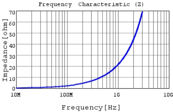
LQP03TN3N4BZ2 |Z|
