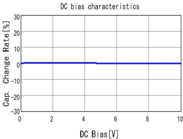
■ GRM21B1X1A104JA01 C-DC bias capchange, 20.0degC, AC1V
