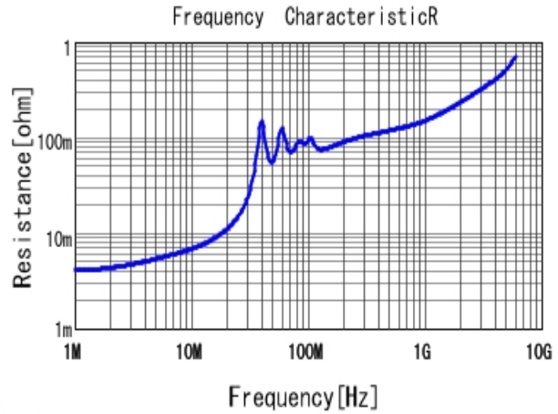
■ GRM21B1X1A104JA01 R DCOV, 20degC
