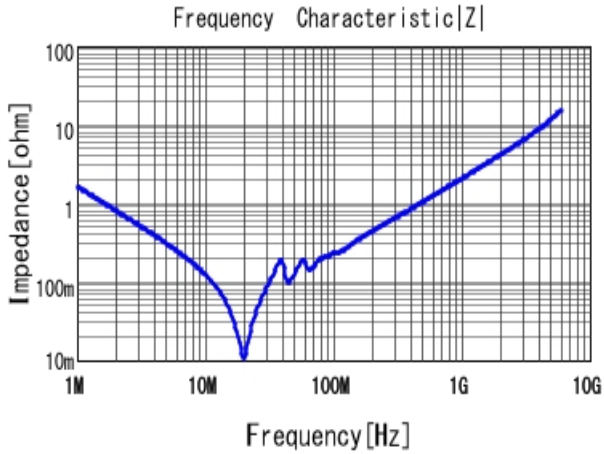
■ GRM21B1X1A104JA01 |Z| DCOV, 20degC
