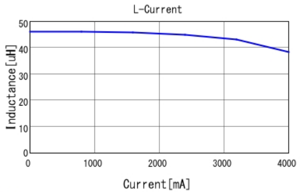
■ MDH12577C-470MA L-Current 20degC
