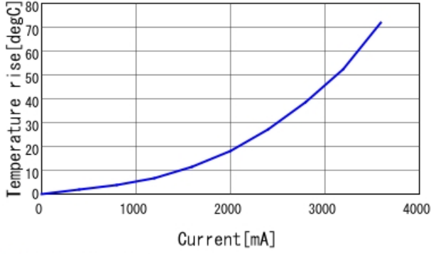
Temperature rise characteristics
