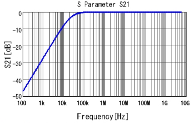
GRM155R71E683KE14 S21 DC0V, 25degC
