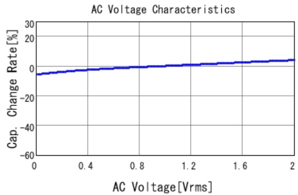
GRM155R71E683KE14 C-AC Voltage capchange, DCOV, 25
