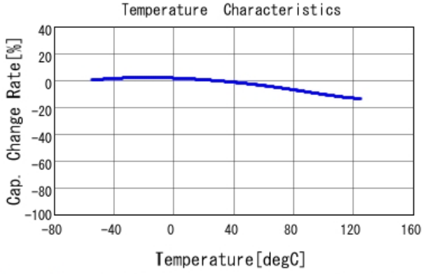
GRM155R71E683KE14 C-Temp. capchange, DC0.0V, AC1.C
