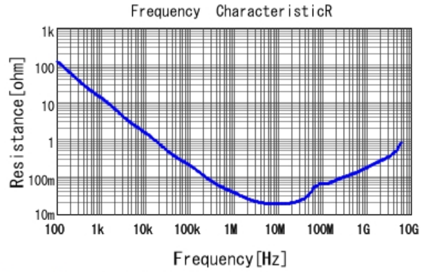
GRM155R71E683KE14 R DCOV, 25degC
