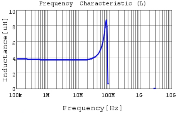
LQH32NZ3R9K23 L
