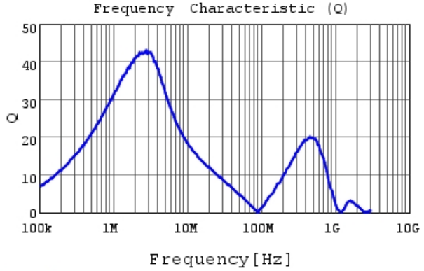
LQH32NZ3R9K23 Q
