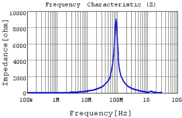
LQH32NZ3R9K23 |Z|
