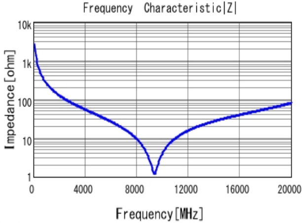
■ GRM1554C1HR60BA01 |Z| DCOV, 20degC
