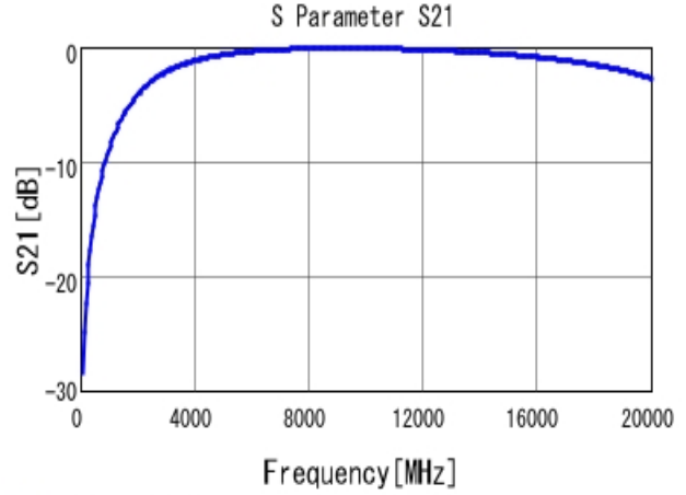
■ GRM1554C1HR60BA01 S21 DCOV, 20degC
