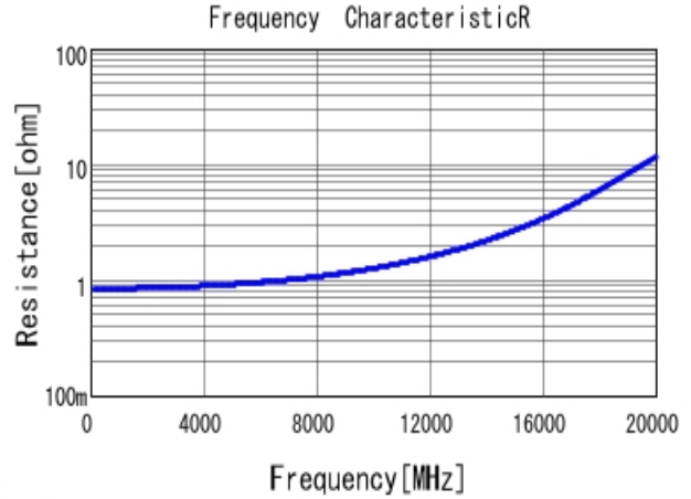
■ GRM1554C1HR60BA01 R DCOV, 20degC
