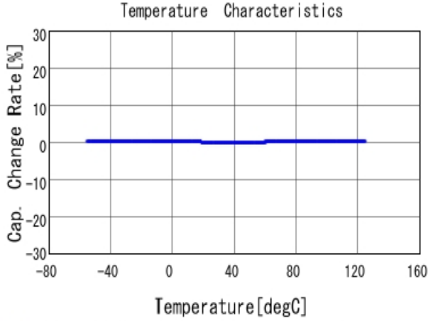
■ GRM1554C1HR60BA01 C-Temp. capchange, DCOV, AC1Vrms
