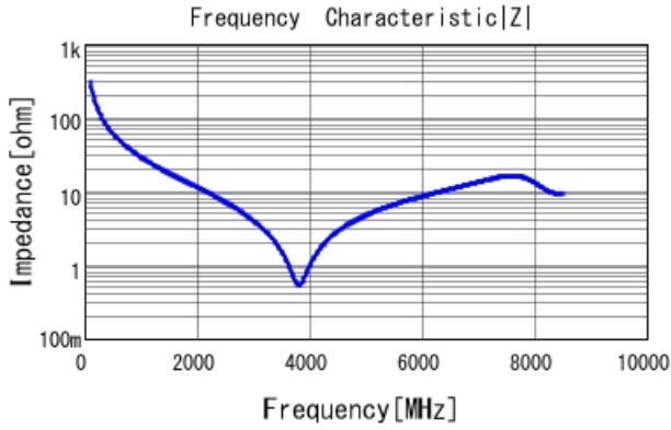
GRM1555C1H5R1CA01 |Z| DCOV, 25degC
