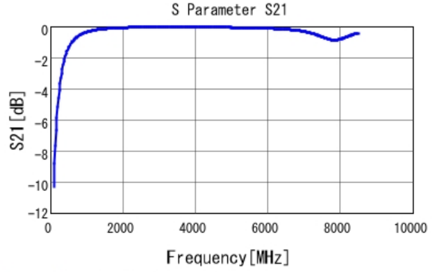
GRM1555C1H5R1CA01 S21 DCOV, 25degC
