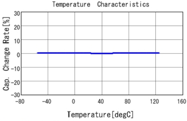
GRM1555C1H5R1CA01 C-Temp. capchange, DCOV, AC1Vrms
