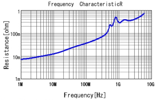
GRM1555C1H122GA01 R DCOV, 25degC
