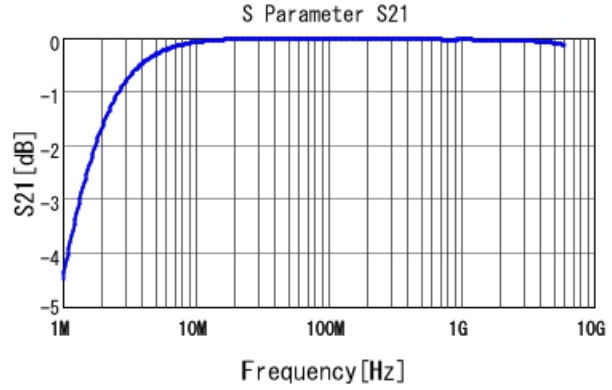
GRM1555C1H122GA01 S21 DCOV, 25degC
