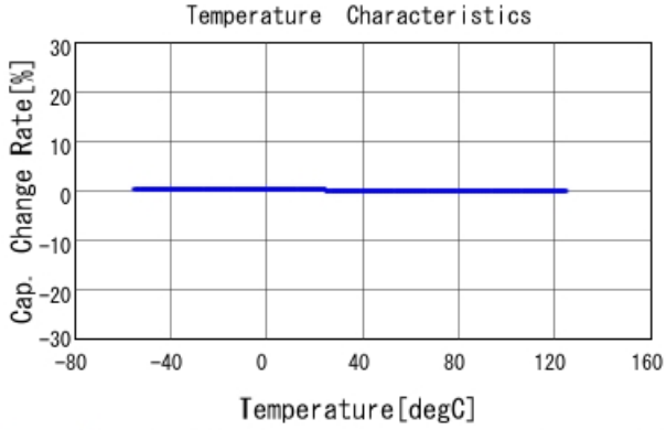
GRM1555C1H122GA01 C-Temp. capchange, DCOV, AC1Vrms
