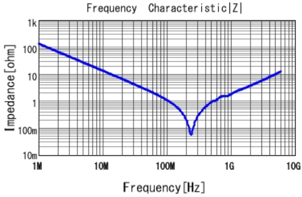
GRM1555C1H122GA01 |Z| DCOV, 25degC
