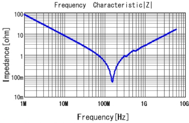
GRM1885C1H202JA01 |Z| DCOV, 25degC
