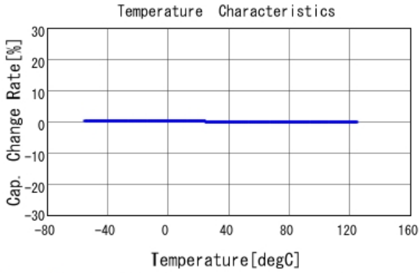
GRM1885C1H202JA01 C-Temp. capchange, DCOV, AC1Vrms
