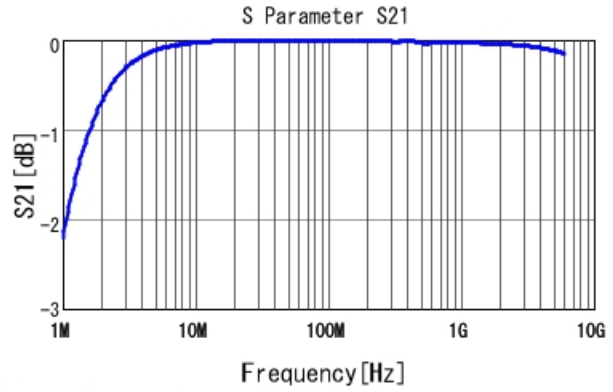
GRM1885C1H202JA01 S21 DCOV, 25degC
