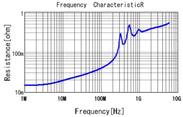
GRM1885C1H202JA01 R DCOV, 25degC
