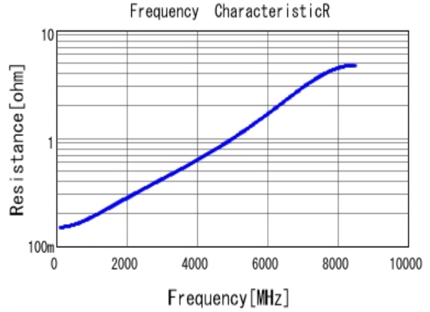
■ GRM0335C1E270JA01 R DC0V, 25degC
