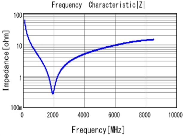
■ GRM0335C1E270JA01 |Z| DC0V, 25degC
