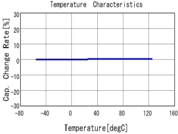
■ GRM1885C1H3R3CA01 C-Temp. capchange, DCOV, AC1Vrms
