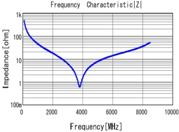
■ GRM1885C1H3R3CA01 |Z| DCOV, 25degC
