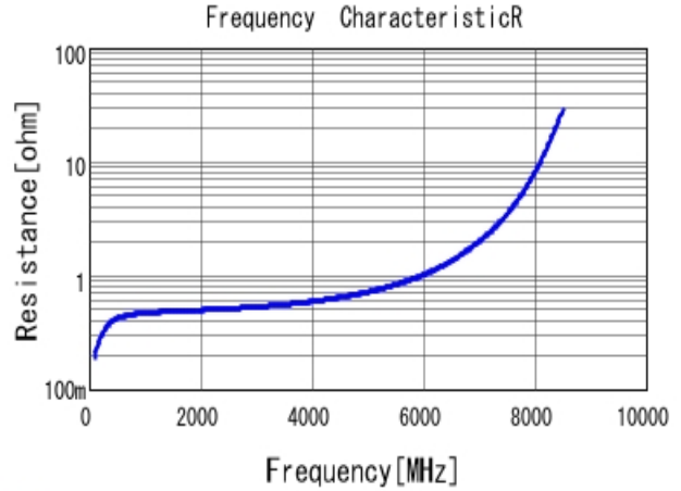
■ GRM1885C1H3R3CA01 R DCOV, 25degC
