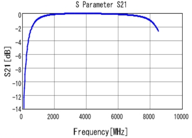
■ GRM1885C1H3R3CA01 S21 DCOV, 25degC
